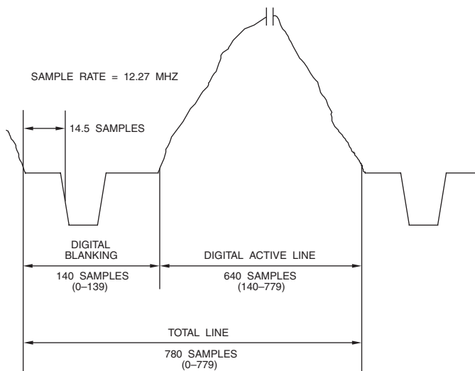
Figure 4.5. 480i Analog-Digital Relationship (4:3 Aspect Ratio, 29.97 Hz Frame Rate, 12.27 MHz Sample Clock).
