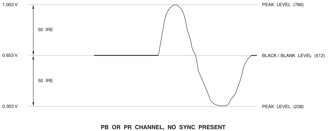
Figure 5.11. EIA-770.3 HDTV Analog YPbPr Levels. Sync on Y.
