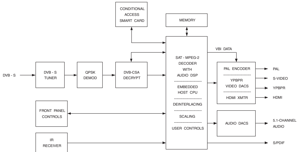
Figure 17.3. DVB Receiver Set-Top Box Block Diagram (Simulcrypt).
