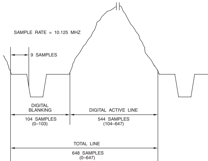
Figure 4.19. 576i Analog-Digital Relationship (4:3 Aspect Ratio, 25 Hz Frame Rate, 10.125 MHz Sample Clock).
