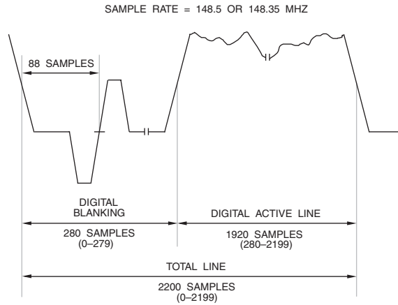
Figure 4.35. 1080p Analog-Digital Relationship (16:9 Aspect Ratio, 59.94 Hz Frame Rate, 148.35 MHz Sample Clock and 60 Hz Frame Rate, 148.5 MHz Sample Clock).
