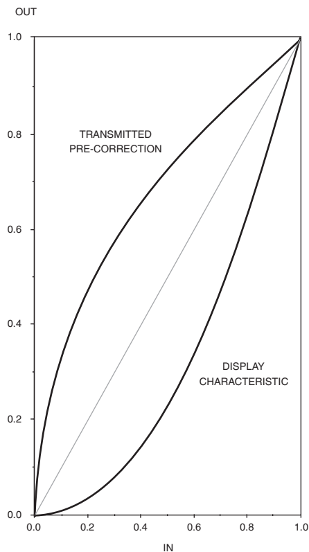
Figure 3.17. Effect of Gamma.
