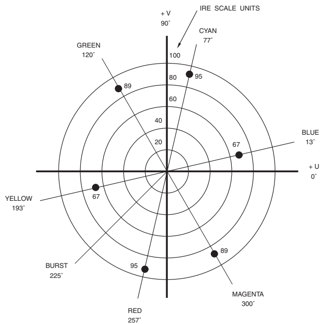
Figure 8.12. UV Vector Diagram for 75% Color Bars. Line [n + 1], PAL switch = 1.
