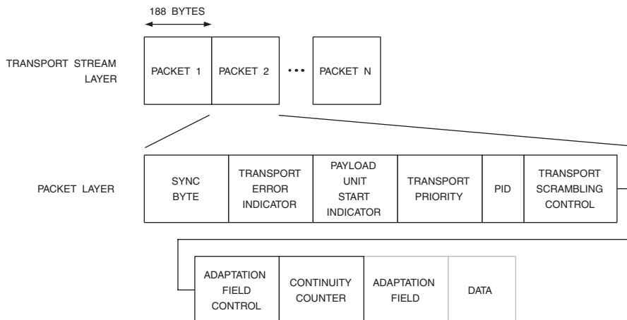
Figure 13.23. MPEG-2 Transport Stream Structure. Marker and reserved bits not shown. Some applications add a 4-byte TP_extra_header prefix (resulting in 192 bytes), consisting of arrival time stamp and copy permission information.
