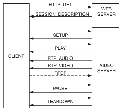
Figure 19.4. Client, Web Server, and Video Server Communications.
