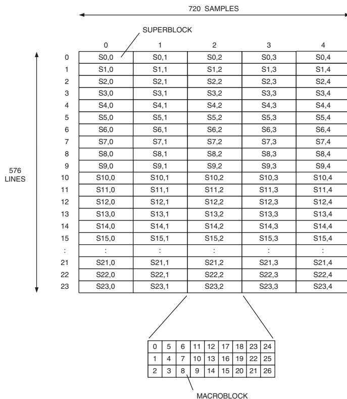
Figure 11.11. Relationship Between Superblocks and Macroblocks (4:2:2 YCbCr, 720 × 576i).
