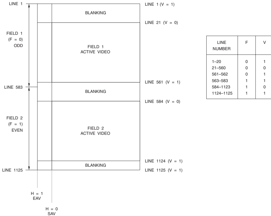
Figure 4.34. 1080i Digital Vertical Timing (1080 Active Lines). F and V change state at the EAV sequence at the beginning of the digital line. Note that the digital line number changes state prior to the start of horizontal sync, as shown in Figures 4.32 and 4.33.
