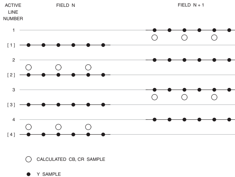
Figure 3.10. 4:2:0 Sampling for MPEG-2, MPEG-4.2, MPEG-4.10 (H.264), and SMPTE 421M (VC-1). The sampling positions on the active scan lines of an interlaced picture (top_field_first = 0).
