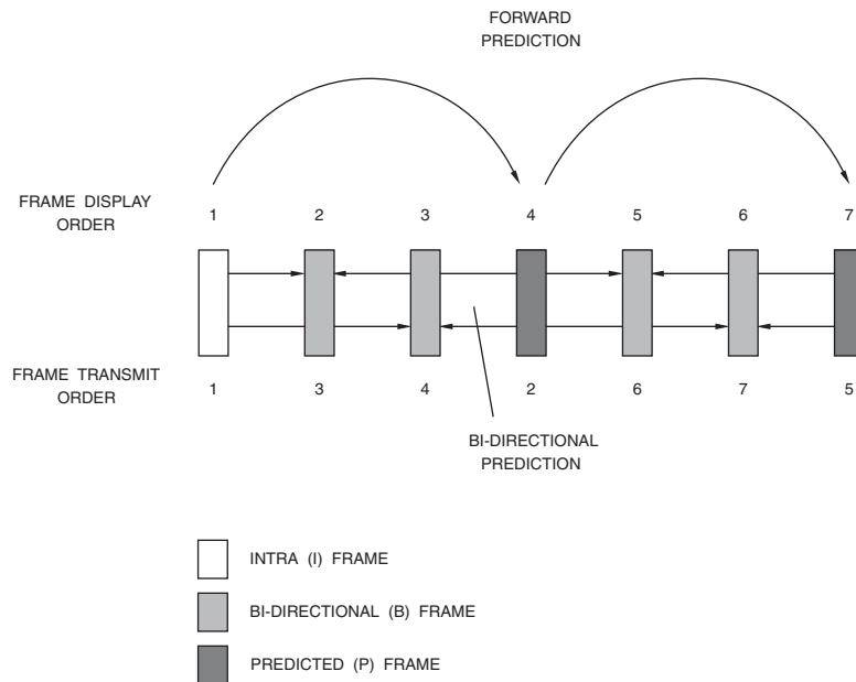
Figure 12.1. MPEG-1 I, P, and B Frames. Some frames are transmitted out of display sequence, complicating the interpolation process, and requiring frame reordering by the MPEG decoder. Arrows show inter-frame dependencies.
