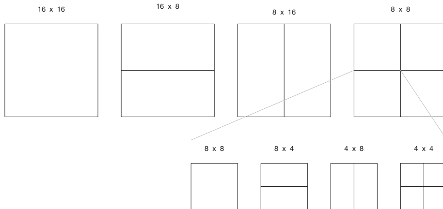
Figure 14.5. Segmentations of H.264 Macroblocks for Motion Compensation. Top: segmentation of macroblocks. Bottom: segmentation of 8 \times 8 partitions.
