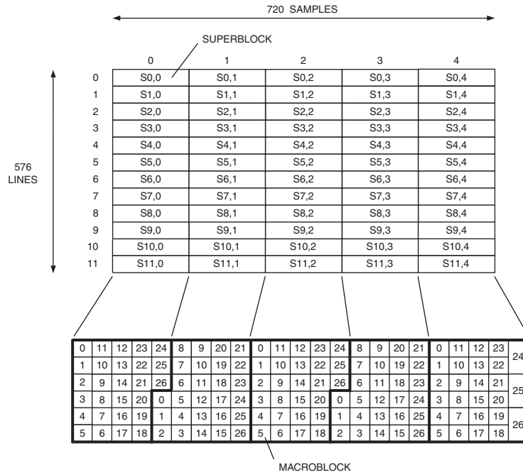
Figure 11.10. Relationship Between Superblocks and Macroblocks (4:1:1 YCbCr, 720 × 576i).
