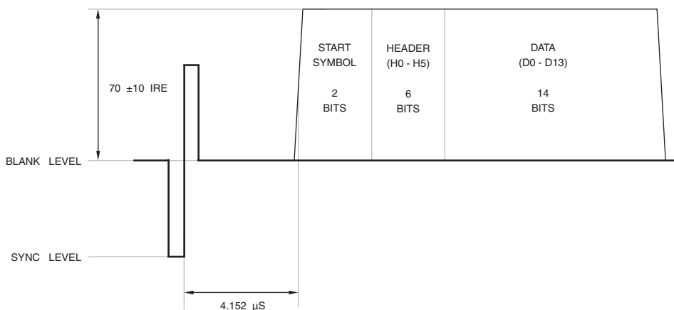
Figure 5.15. CEA-805 and EIA-J CPR-1204-2 Lines 19 and 582 Timing.
