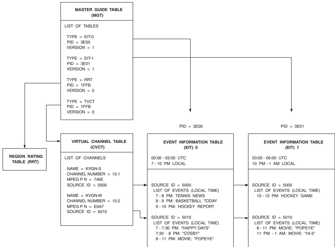
Figure 16.1. OpenCable™ In-Band SI Table Relationships.
