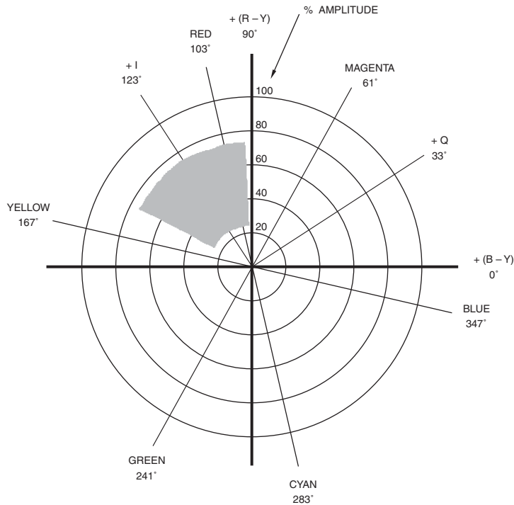
Figure 9.28. Typical Skin Tone Color Range.
