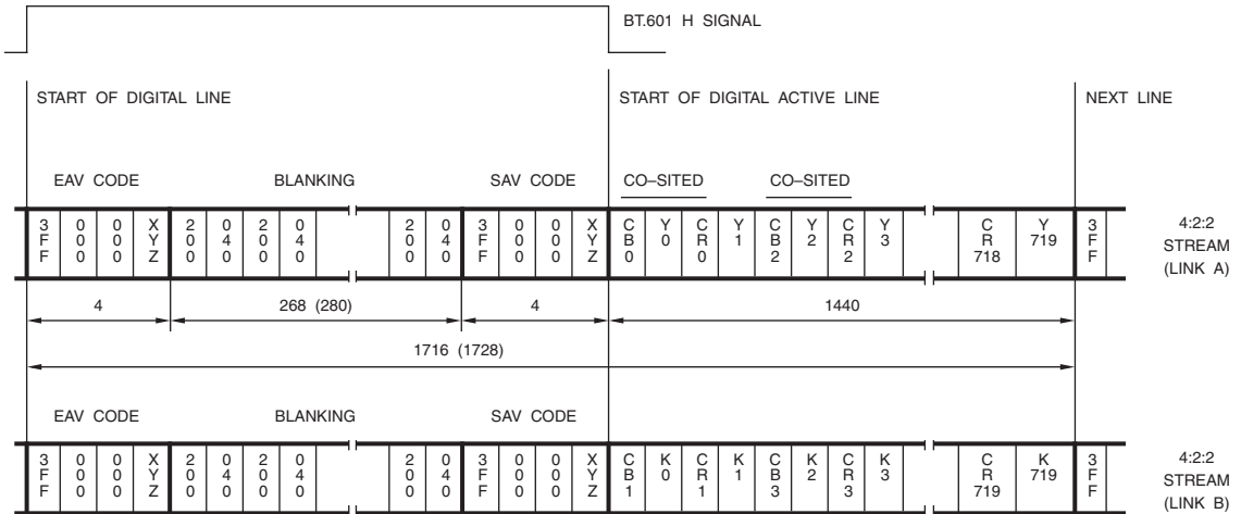
Figure 6.10. BT.799 and SMPTE RP-175 Parallel Interface Data for One Scan Line. 480i; 4:4:4:4 YCbCrK; 720 active samples per line; 27 MHz clock; 10-bit system. The values for 576i systems are shown in parentheses.
