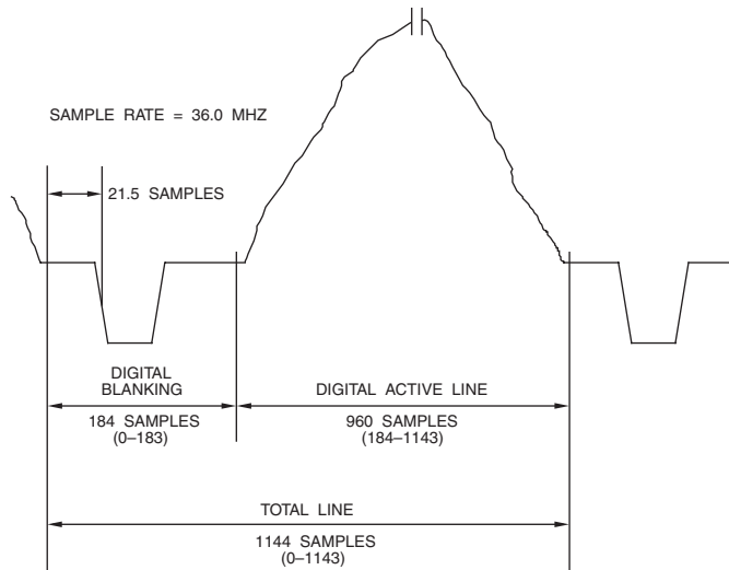
Figure 4.10. 480p Analog-Digital Relationship (16:9 Aspect Ratio, 59.94 Hz Frame Rate, 36 MHz Sample Clock).
