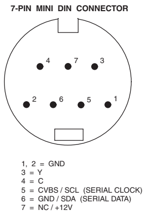
Figure 5.1. S-Video Connector and Signal Names.
