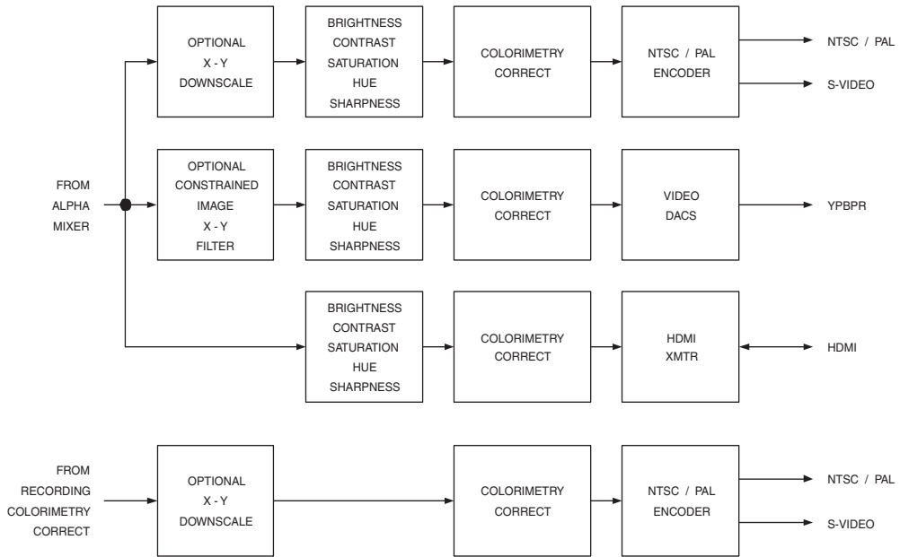
Figure 7.63. Video Output Port Processing.
