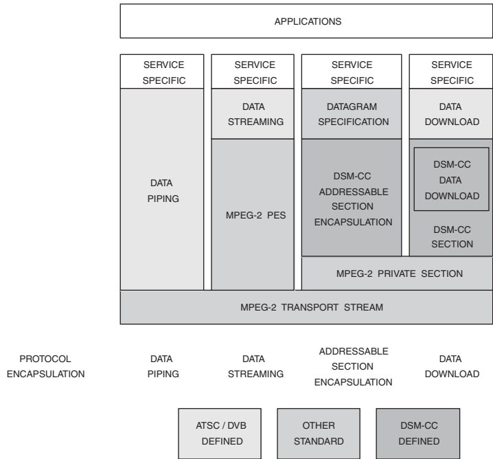
Figure 13.29. Encapsulation Overview.
