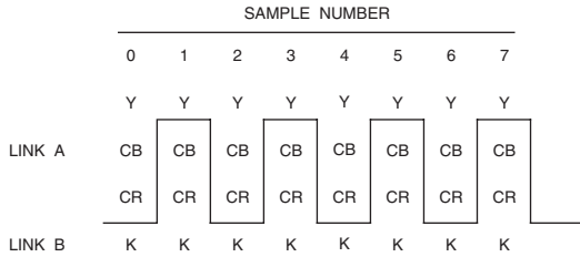
Figure 6.8. Link Content Representation for YCbCrK Video Signals.
