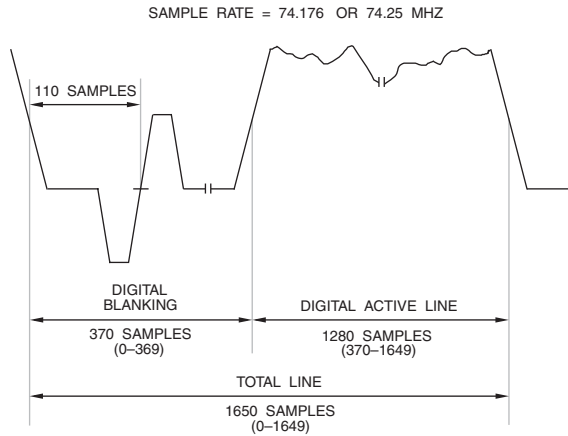
Figure 4.27. 720p Analog-Digital Relationship (16:9 Aspect Ratio, 59.94 Hz Frame Rate, 74.176 MHz Sample Clock and 60 Hz Frame Rate, 74.25 MHz Sample Clock).
