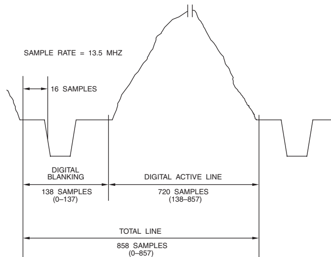
Figure 4.3. 480i Analog-Digital Relationship (4:3 Aspect Ratio, 29.97 Hz Frame Rate, 13.5 MHz Sample Clock). BT.601 specifies 16 samples for the front porch; CEA-861D (DVI and HDMI timing) specifies 19 samples for the front porch.
