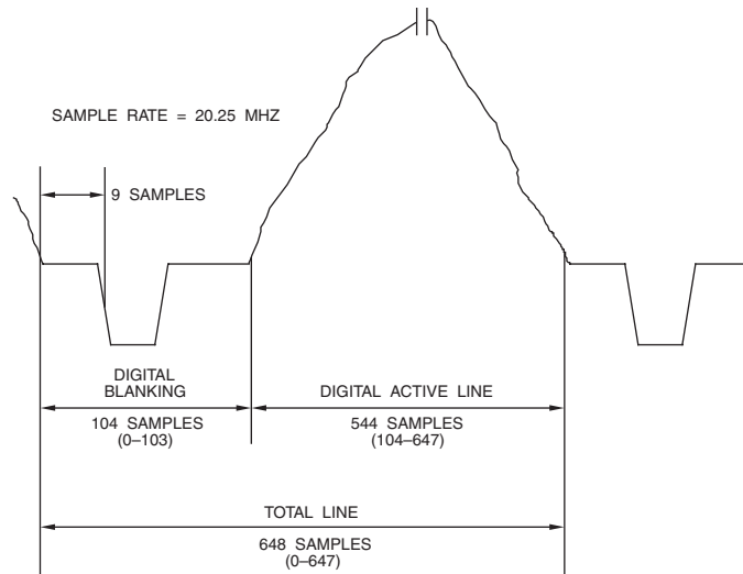
Figure 4.24. 576p Analog-Digital Relationship (4:3 Aspect Ratio, 50 Hz Frame Rate, 20.25 MHz Sample Clock).
