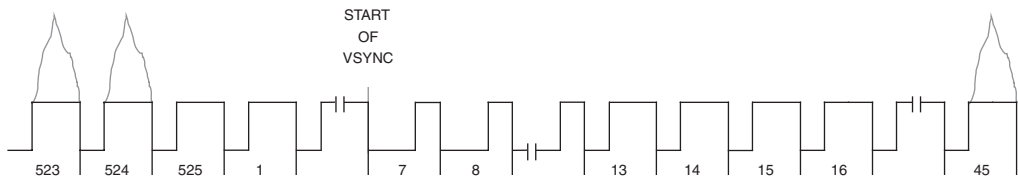
Figure 4.2. 480p Vertical Interval Timing.
