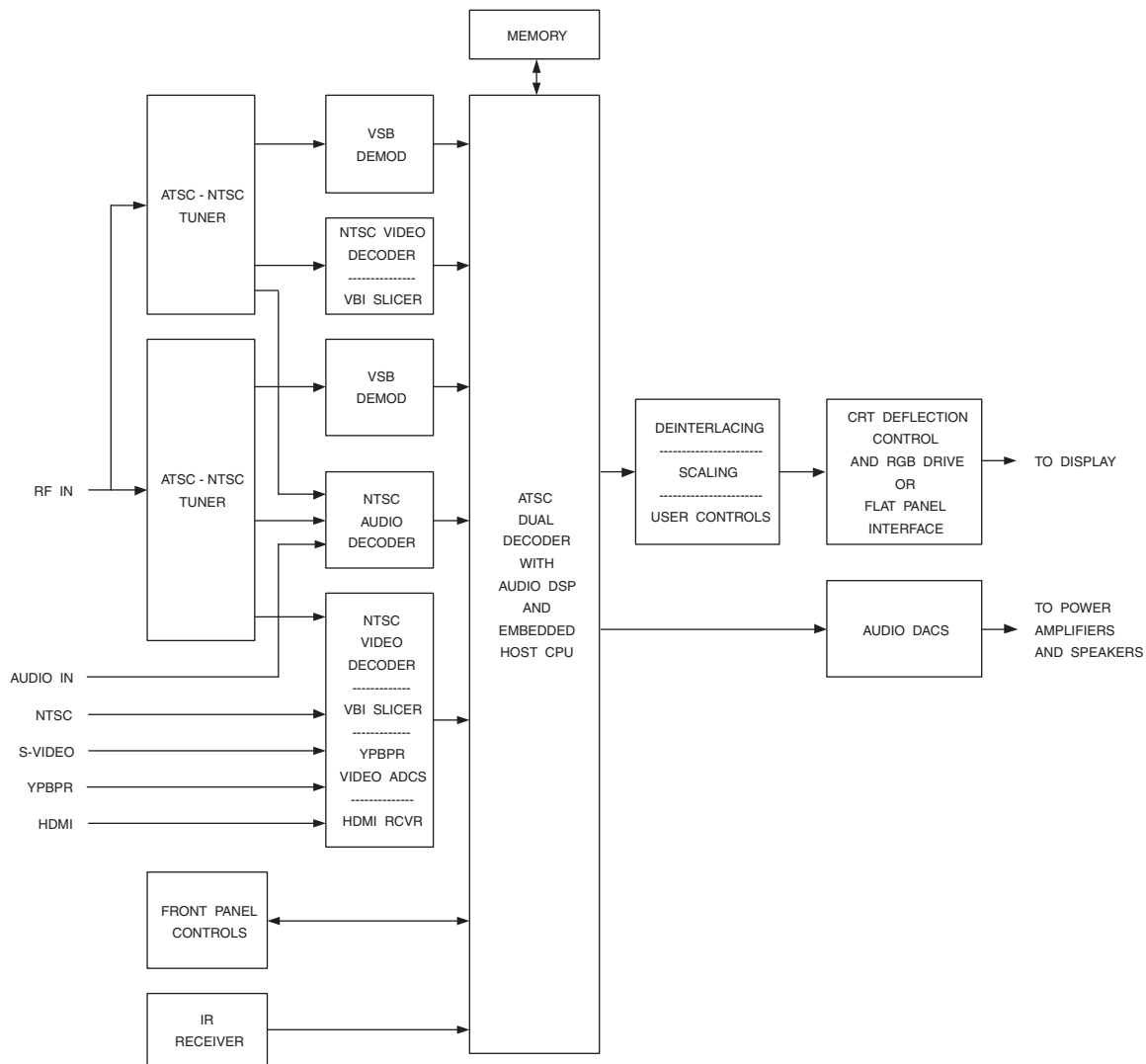
Figure 15.3. Typical ATSC Digital Television Block Diagram.
