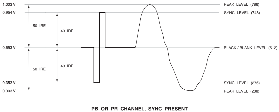
Figure 5.12. SMPTE 274M and 296M HDTV Analog YPbPr Levels. Sync on YPbPr.
