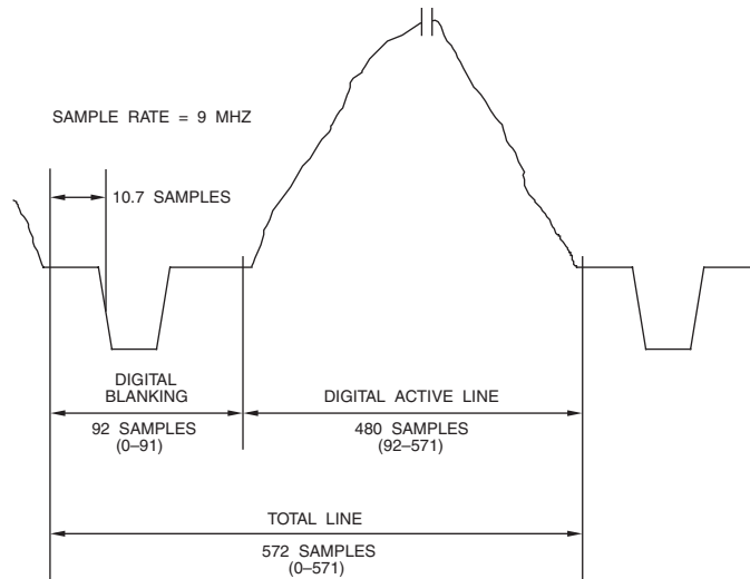
Figure 4.7. 480i Analog-Digital Relationship (4:3 Aspect Ratio, 29.97 Hz Frame Rate, 9 MHz Sample Clock).
