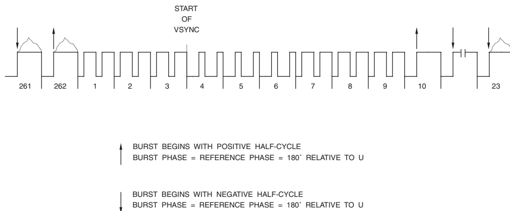
Figure 8.7. Noninterlaced NTSC Frame Sequence.
