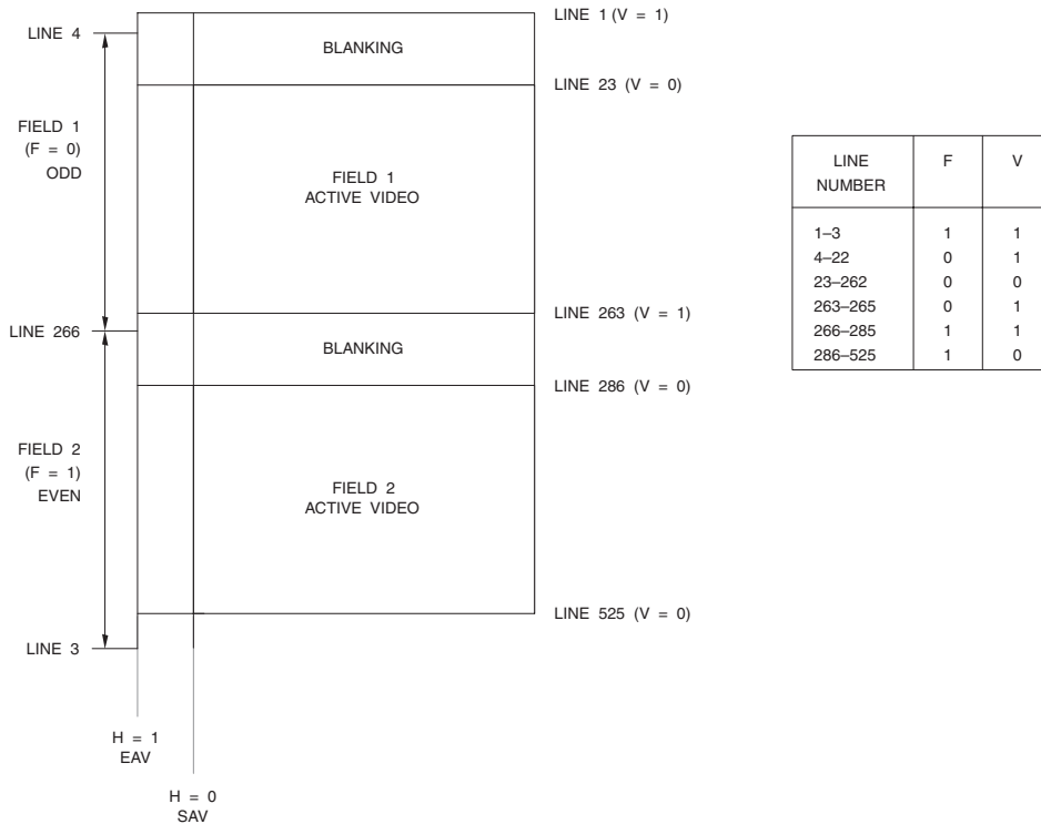
Figure 4.8. 480i Digital Vertical Timing (480 Active Lines). F and V change state at the EAV sequence at the beginning of the digital line. Note that the digital line number changes state prior to the start of horizontal sync, as shown in Figures 4.3 through 4.7.
