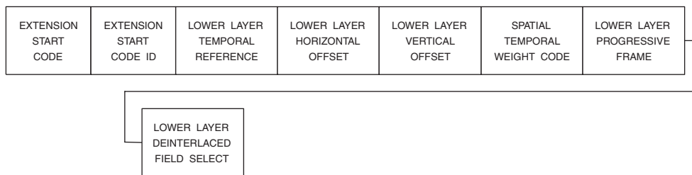
Figure 13.13. MPEG-2 Picture Spatial Scalable Extension Structure. Marker bits not shown.
