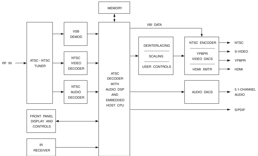
Figure 15.2. Typical ATSC Receiver Set-Top Box Block Diagram.
