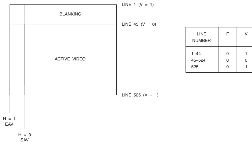
Figure 4.13. 480p Digital Vertical Timing (480 Active Lines). V changes state at the EAV sequence at the beginning of the digital line. Note that the digital line number changes state prior to the start of horizontal sync, as shown in Figures 4.9 through 4.12.
