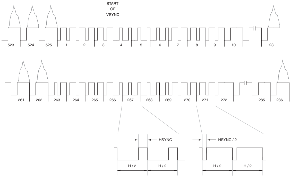
Figure 4.1. 480i Vertical Interval Timing.
