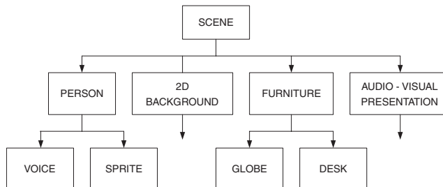
Figure 14.3. Example MPEG-4 Hierarchical Scene Graph.
