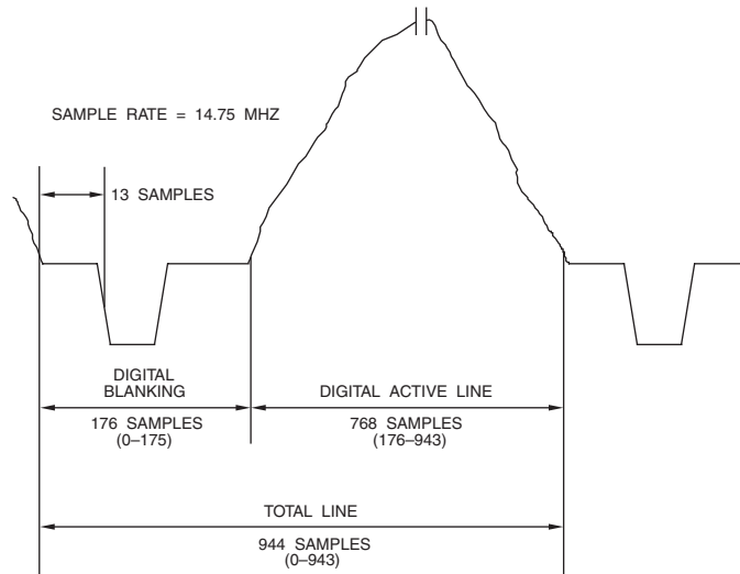
Figure 4.18. 576i Analog-Digital Relationship (4:3 Aspect Ratio, 25 Hz Frame Rate, 14.75 MHz Sample Clock).
