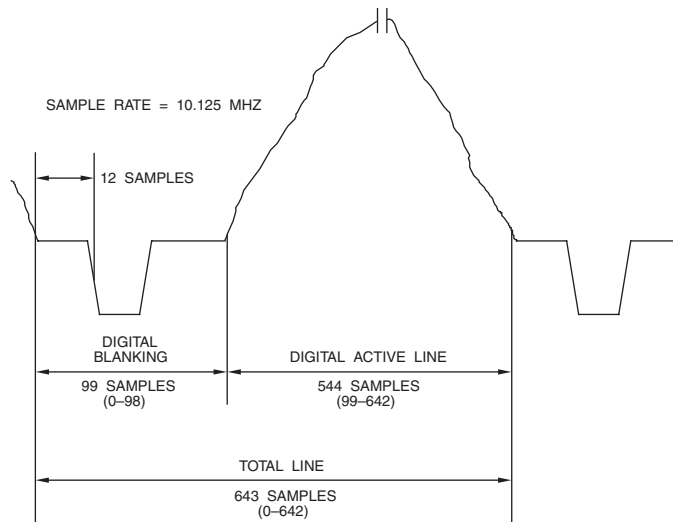
Figure 4.6. 480i Analog-Digital Relationship (4:3 Aspect Ratio, 29.97 Hz Frame Rate, 10.125 MHz Sample Clock).
