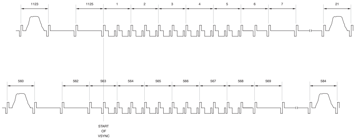
Figure 4.30. 1080i Vertical Interval Timing.
