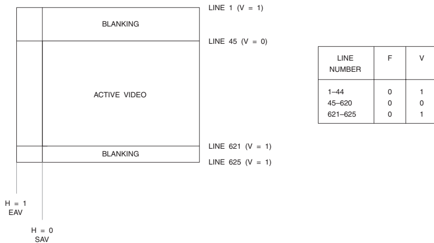
Figure 4.25. 576p Digital Vertical Timing (576 Active Lines). V changes state at the EAV sequence at the beginning of the digital line. Note that the digital line number changes state prior to the start of horizontal sync, as shown in Figures 4.21 through 4.24.
