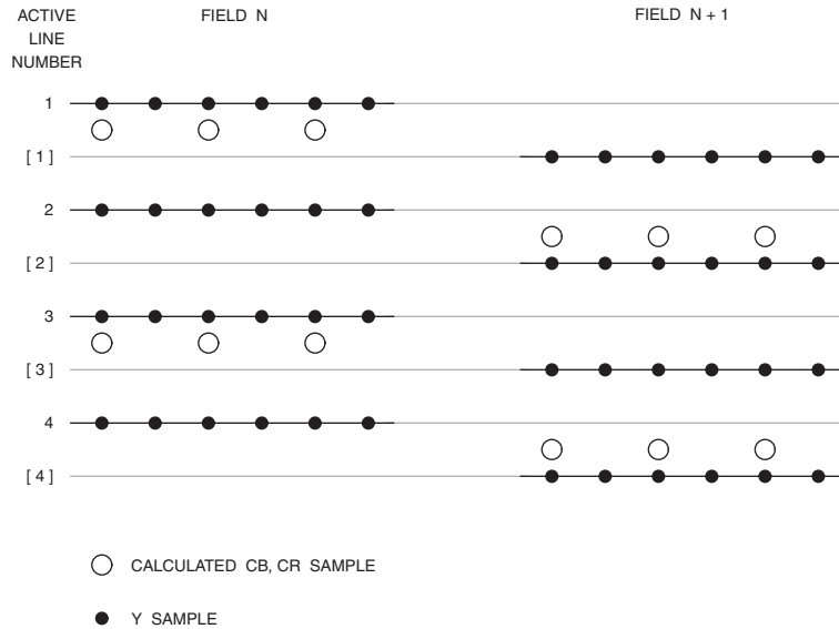
Figure 3.9. 4:2:0 Sampling for MPEG-2, MPEG-4.2, MPEG-4.10 (H.264), and SMPTE 421M (VC-1). The sampling positions on the active scan lines of an interlaced picture (top_field_first = 1).
