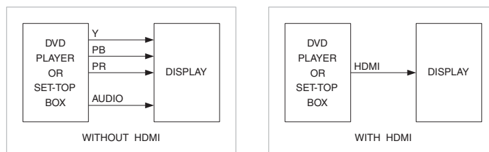
Figure 6.48. Using HDMI Eliminates Confusing Cable Connections for Consumers.
