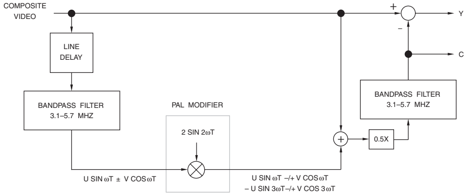
Figure 9.38. Single-Line Delay PAL Y/C Separator Using a PAL Modifier.
