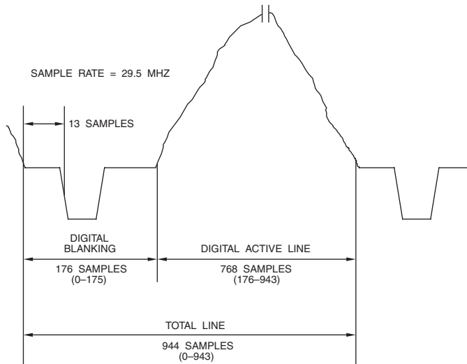
Figure 4.23. 576p Analog-Digital Relationship (4:3 Aspect Ratio, 50 Hz Frame Rate, 29.5 MHz Sample Clock).
