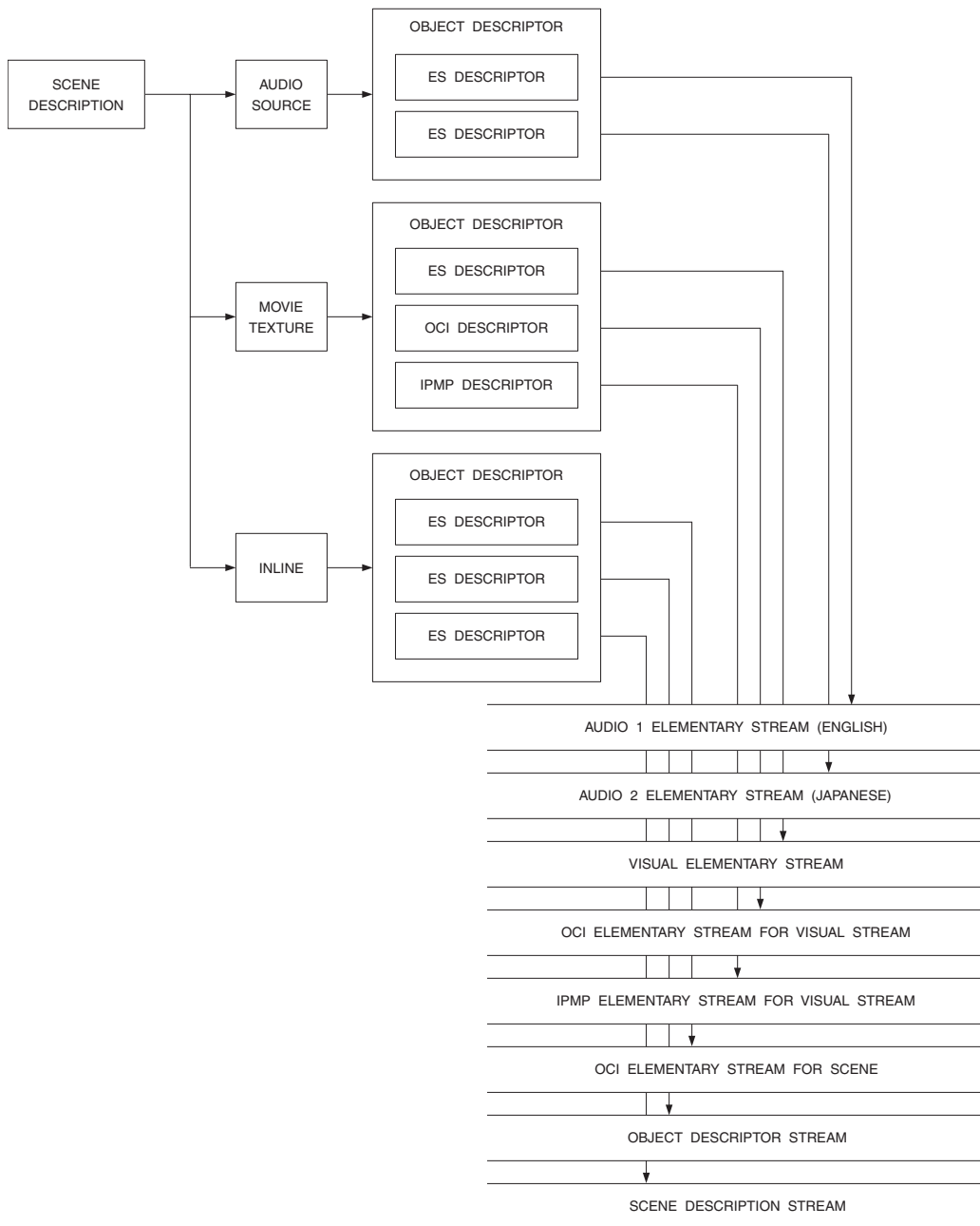
Figure 14.2. Linking Elementary Streams to a Scene.
