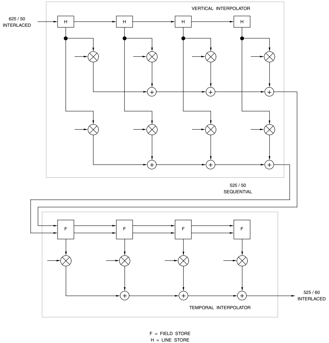
Figure 7.41. Typical 50 Hz to 60 Hz Conversion Using Vertical, Followed by Temporal, Interpolation.
