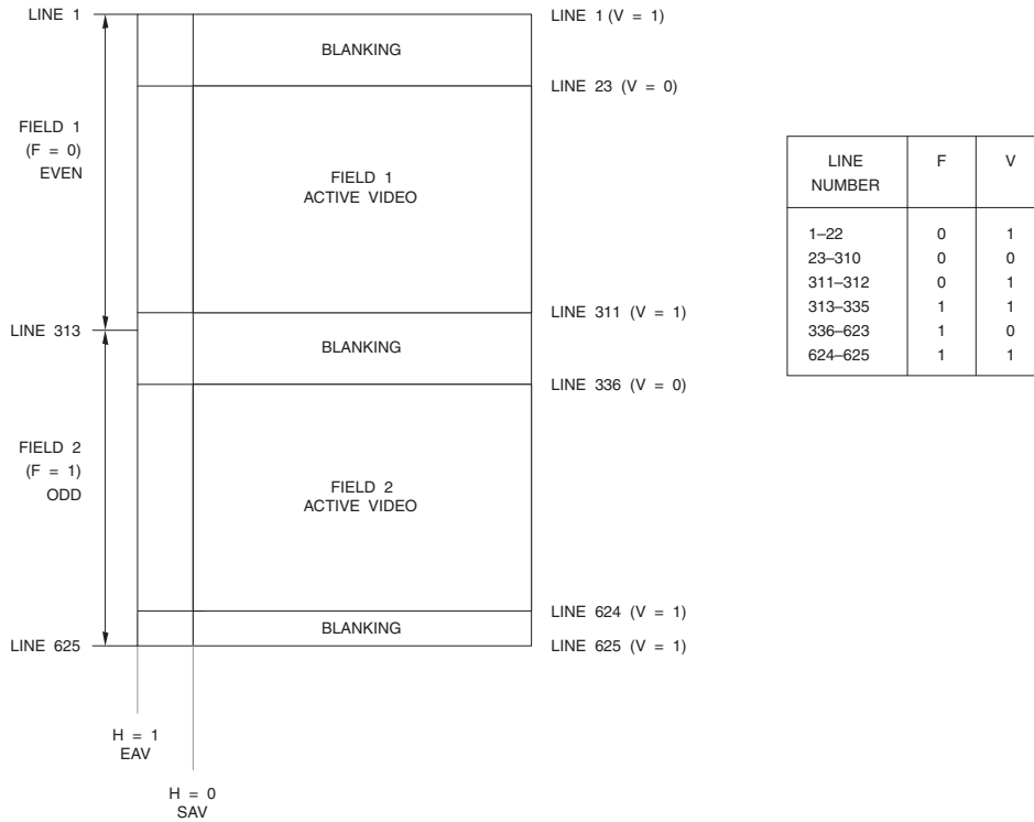
Figure 4.20. 576i Digital Vertical Timing (576 Active Lines). F and V change state at the EAV sequence at the beginning of the digital line. Note that the digital line number changes state prior to the start of horizontal sync, as shown in Figures 4.16 through 4.19.
