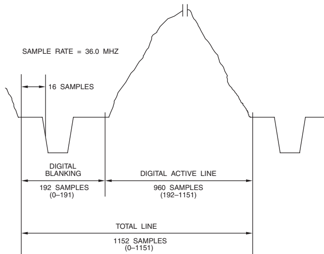
Figure 4.22. 576p Analog-Digital Relationship (16:9 Aspect Ratio, 50 Hz Frame Rate, 36 MHz Sample Clock).
