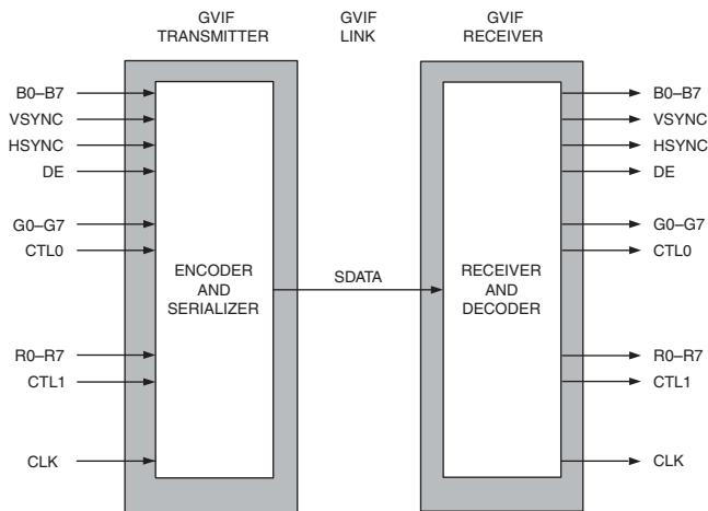
Figure 6.52. GVIF Link.
