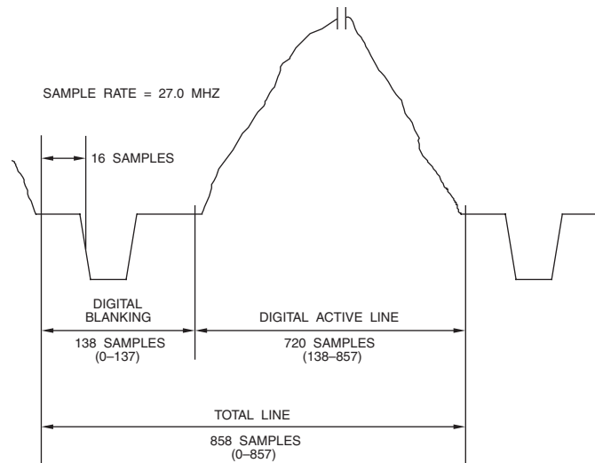
Figure 4.9. 480p Analog-Digital Relationship (4:3 Aspect Ratio, 59.94 Hz Frame Rate, 27 MHz Sample Clock).
