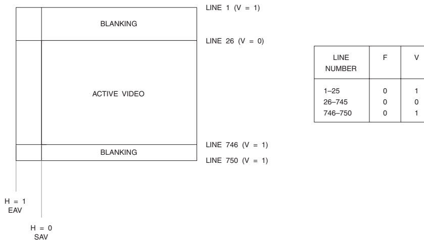
Figure 4.29. 720p Digital Vertical Timing (720 Active Lines). V changes state at the EAV sequence at the beginning of the digital line. Note that the digital line number changes state prior to the start of horizontal sync, as shown in Figures 4.27 and 4.28.
