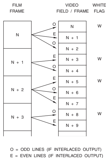
Figure 7.46. 3:2 Pulldown for Converting 24 Hz Film to 60 Hz Video.
