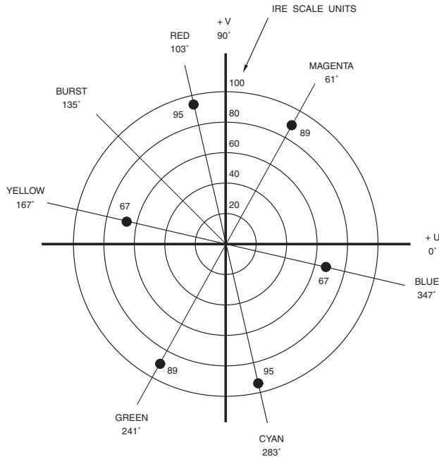
Figure 8.11. UV Vector Diagram for 75% Color Bars. Line [n], PAL switch = 0.
