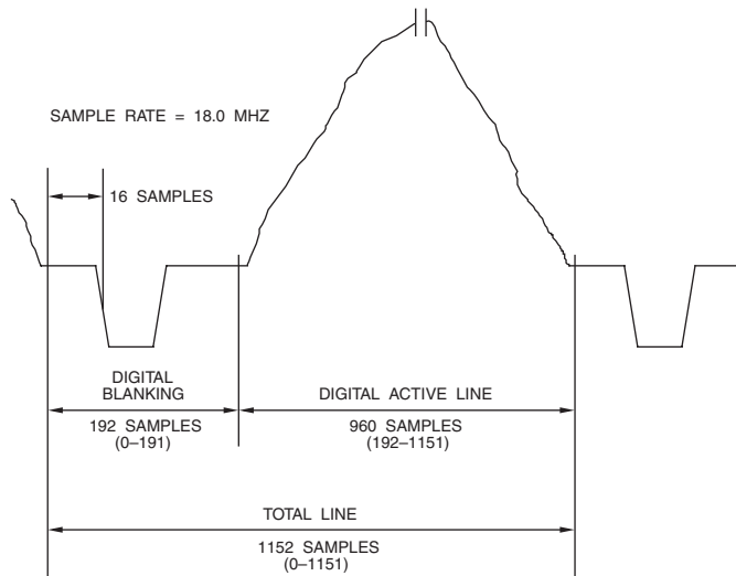
Figure 4.17. 576i Analog-Digital Relationship (16:9 Aspect Ratio, 25 Hz Frame Rate, 18 MHz Sample Clock).
