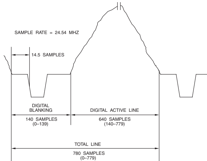
Figure 4.11. 480p Analog-Digital Relationship (4:3 Aspect Ratio, 59.94 Hz Frame Rate, 24.54 MHz Sample Clock).
