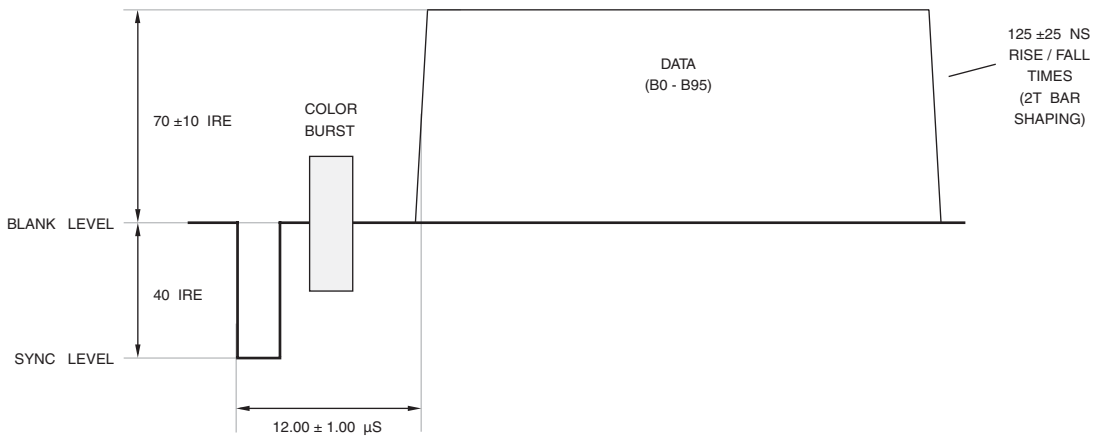
Figure 8.65. 525-Line Lines 20, 22, 283, and 284 AMOL II Timing.
