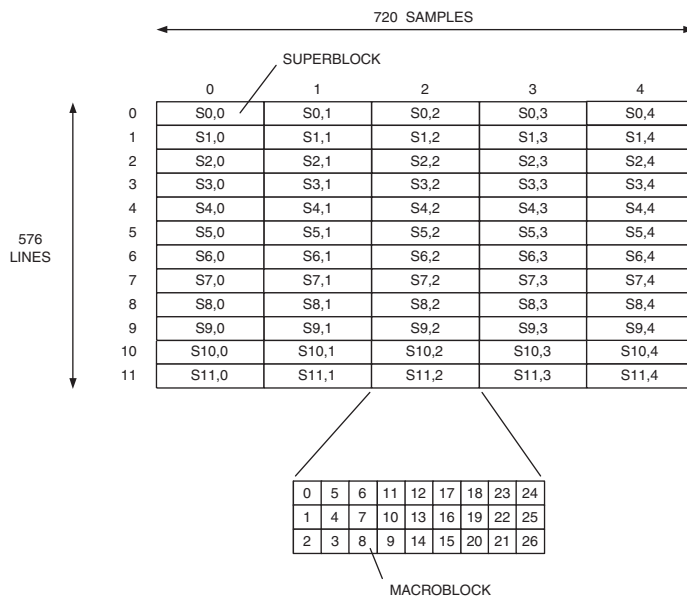
Figure 11.9. Relationship Between Superblocks and Macroblocks (4:2:0 YCbCr, 720 × 576i).
