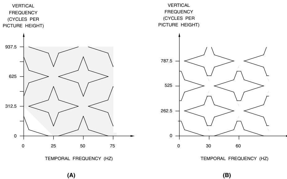
Figure 7.44. Spectral Representation of Combined Vertical and Temporal Interpolation. (A) Two-dimensional lowpass filtering. (B) Resampling to final standard.
