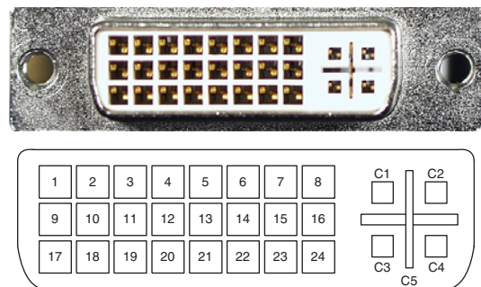
Figure 6.47. DVI-I Connector.
