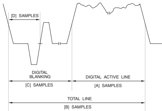
Figure 4.33. General 1080i Analog-Digital Relationship.
