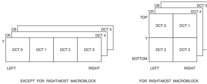
Figure 11.5. 4:1:1 Macroblock Arrangement.
