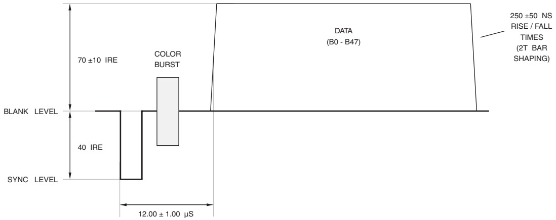
Figure 8.64. 525-Line Lines 20, 22, 283, and 284 AMOL I Timing.
