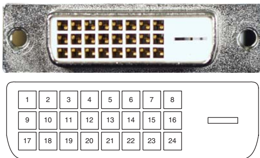
Figure 6.46. DVI-D Connector.
