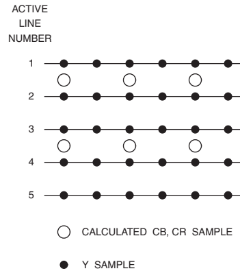
Figure 3.8. 4:2:0 Sampling for MPEG-2, MPEG-4.2, MPEG-4.10 (H.264), and SMPTE 421M (VC-1). The sampling positions on the active scan lines of a progressive or noninterlaced picture.
