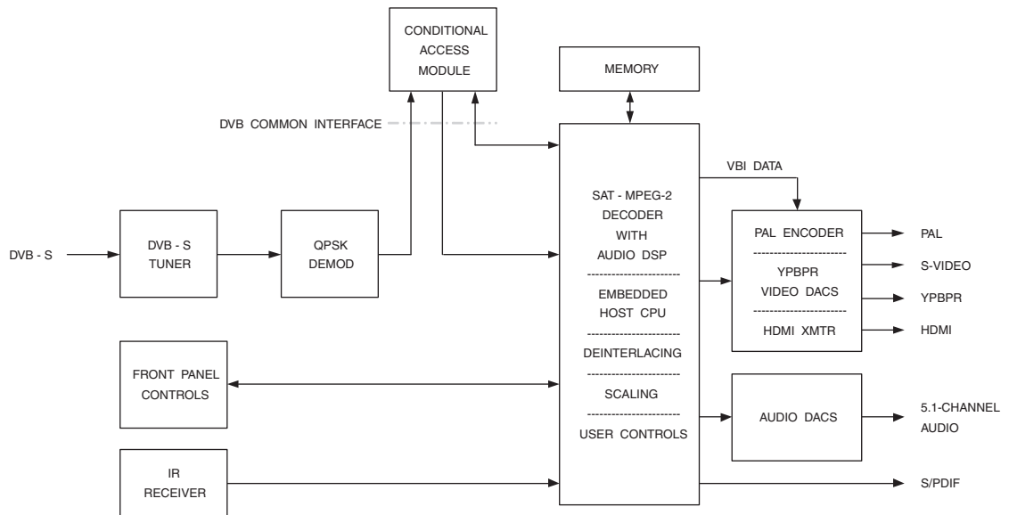
Figure 17.2. DVB Receiver Set-Top Box Block Diagram (Multicrypt).
