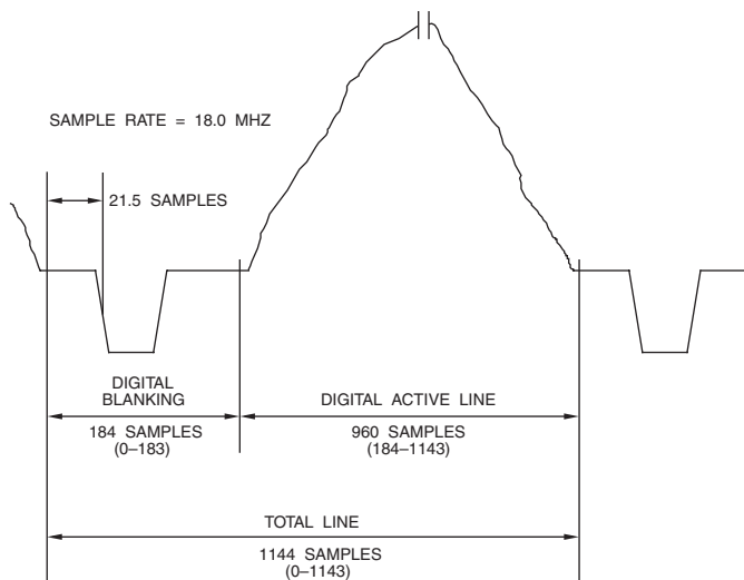
Figure 4.4. 480i Analog-Digital Relationship (16:9 Aspect Ratio, 29.97 Hz Frame Rate, 18 MHz Sample Clock).
