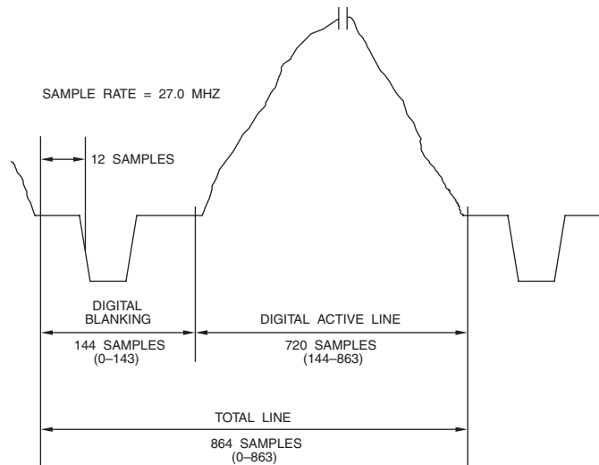
Figure 4.21. 576p Analog-Digital Relationship (4:3 Aspect Ratio, 50 Hz Frame Rate, 27 MHz Sample Clock).
