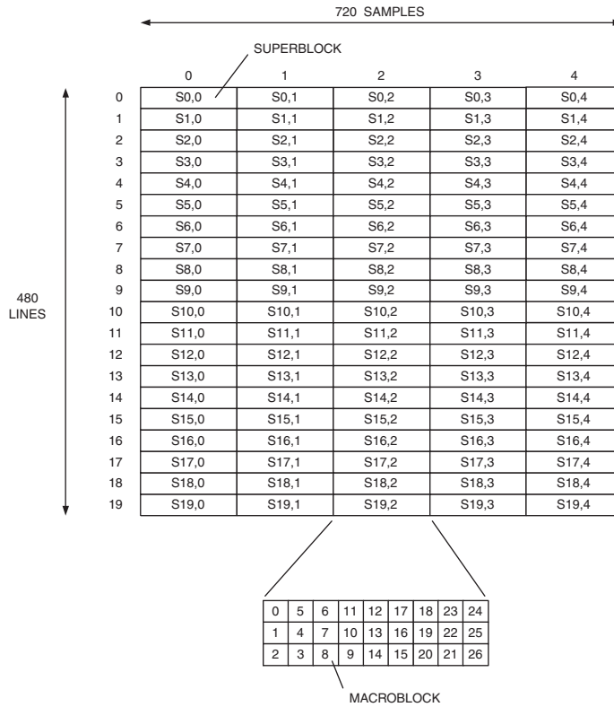
Figure 11.8. Relationship Between Superblocks and Macroblocks (4:2:2 YCbCr, 720 × 480i).
