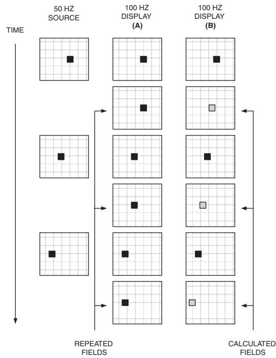
Figure 7.45. 50 Hz to 100 Hz (Double Scan Interlaced) Techniques.
