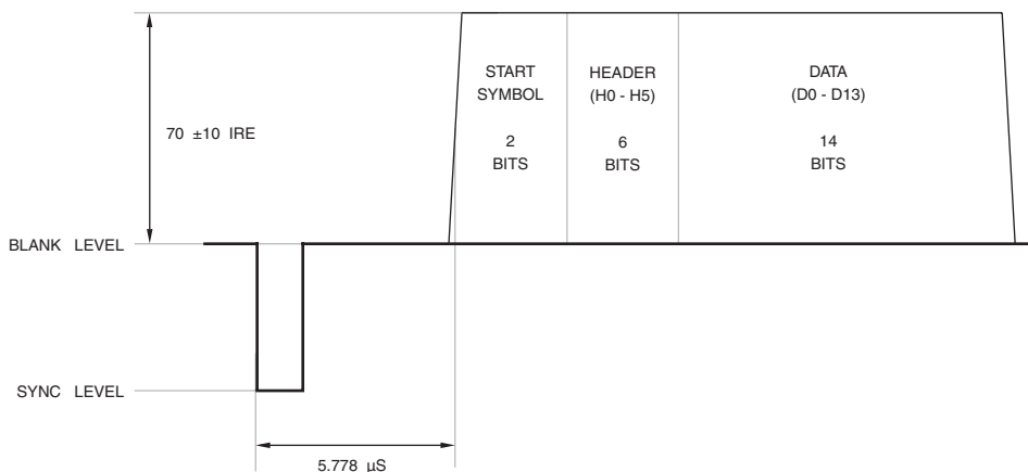
Figure 5.8. CEA-805, IEC 61880–2, and EIA-J CPR-1204–1 Line 41 Timing.
