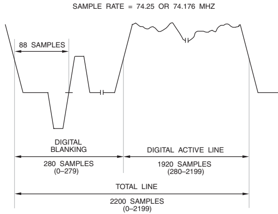
Figure 4.32. 1080i Analog-Digital Relationship (16:9 Aspect Ratio, 29.97 Hz Frame Rate, 74.176 MHz Sample Clock and 30 Hz Frame Rate, 74.25 MHz Sample Clock).
