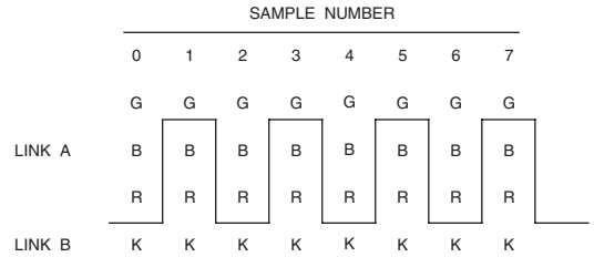
Figure 6.9. Link Content Representation for R'G'B'K Video Signals.
