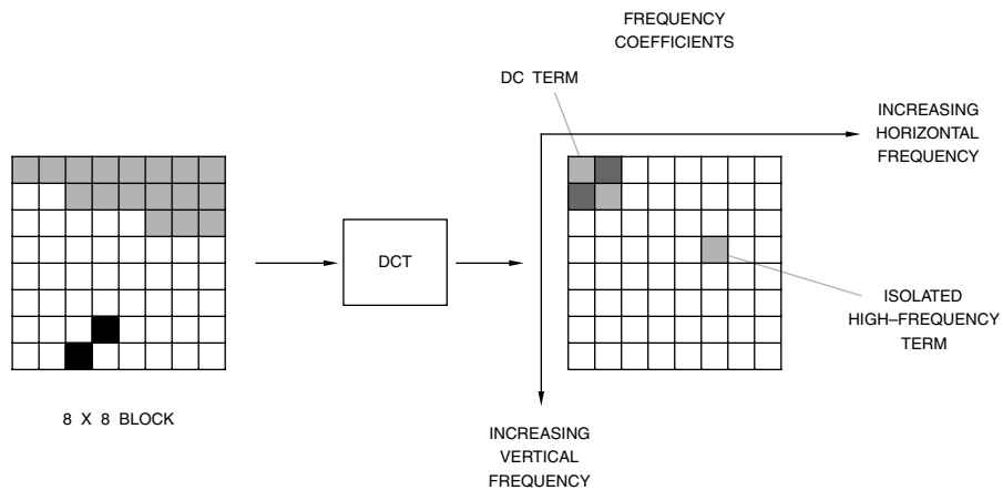
Figure 7.56. The DCT Processes the 8 \times 8 Block of Samples or Error Terms to Generate an 8 \times 8 Block of DCT Coefficients.
