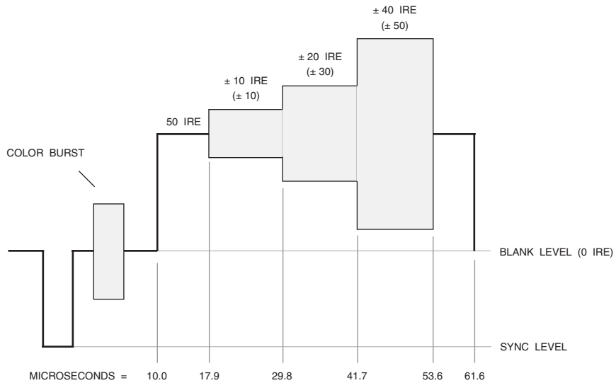
Figure 8.36. Modulated Pedestal Test Signal for NTSC and PAL. PAL IRE values are shown in parentheses.
