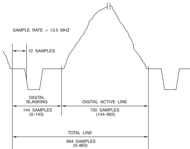
Figure 4.16. 576i Analog-Digital Relationship (4:3 Aspect Ratio, 25 Hz Frame Rate, 13.5 MHz Sample Clock).
