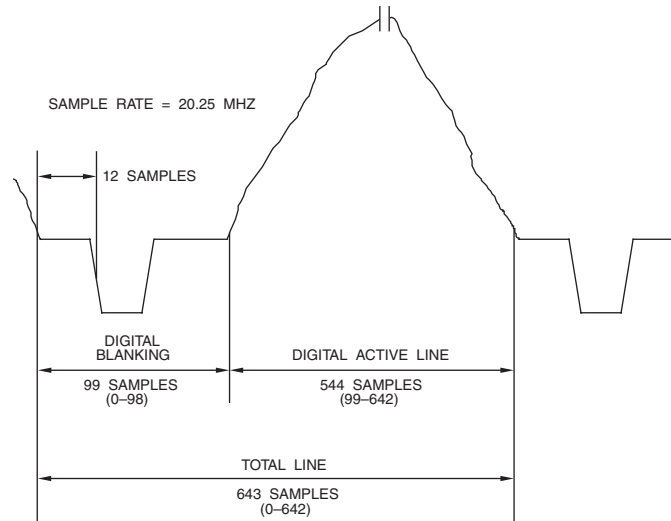
Figure 4.12. 480p Analog-Digital Relationship (4:3 Aspect Ratio, 59.94 Hz Frame Rate, 20.25 MHz Sample Clock).
