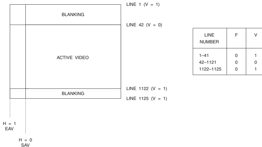
Figure 4.37. 1080p Digital Vertical Timing (1080 Active Lines). V changes state at the EAV sequence at the beginning of the digital line. Note that the digital line number changes state prior to the start of horizontal sync, as shown in Figures 4.35 and 4.36.
