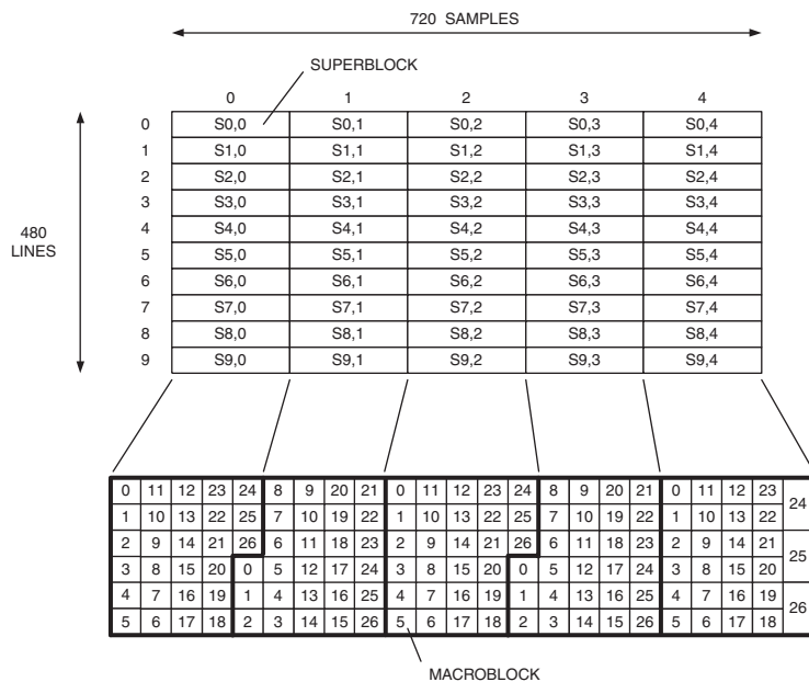
Figure 11.7. Relationship Between Superblocks and Macroblocks (4:1:1 YCbCr, 720 × 480i).
