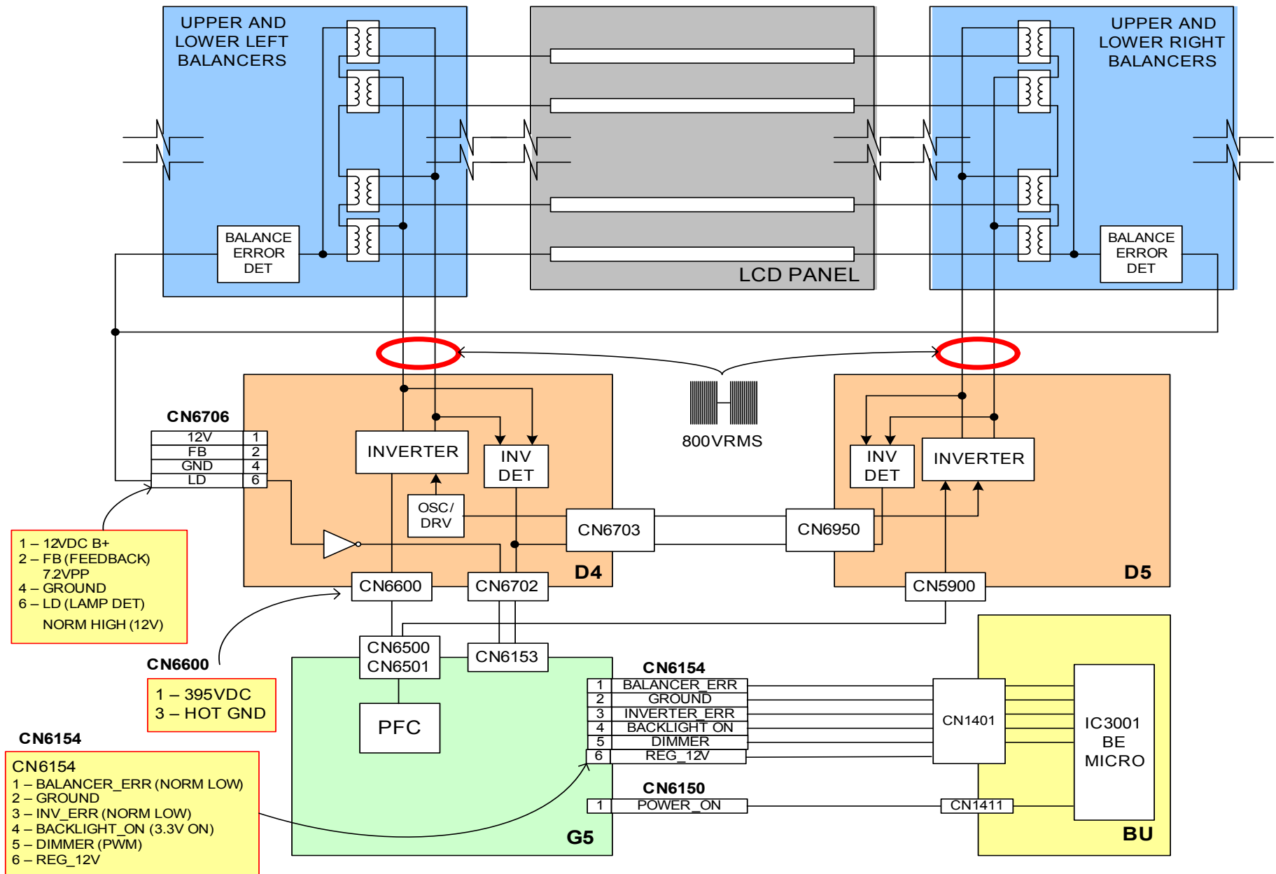
FIGURE 6-7 52-INCH PANEL BACKLIGHT DIAGRAM
