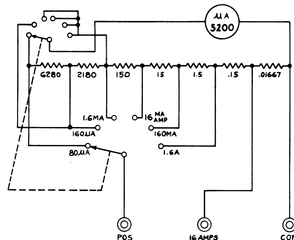
FIGURE 8. MODEL 262 CIRCUIT FOR DC CURRENT MEASUREMENTS
