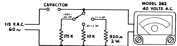
FIGURE 10. CIRCUIT USED TO MEASURE CAPACITY WITH THE MODEL 262
